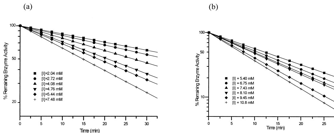
Figure 2. Loss of enzyme activity of CPA as a function of incubation time.
