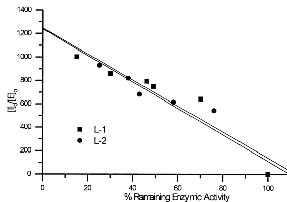
Figure 6. Determination of partition ratio by the titration method.
