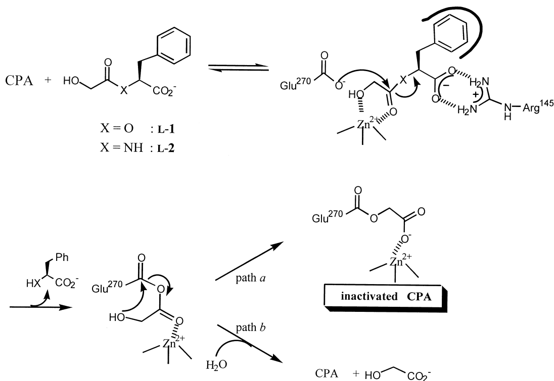
Figure 1. Schematic illustration of the rationale used for designing L-1 and L-2 as mechanism-based inactivators for CPA.
