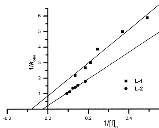
Figure 4. Double reciprocal plot of k_{\text{obs}} versus [\text{inactivator}]_0 . Values of k_{\text{inact}} and K_I were calculated from y intercept and the slope, respectively.
