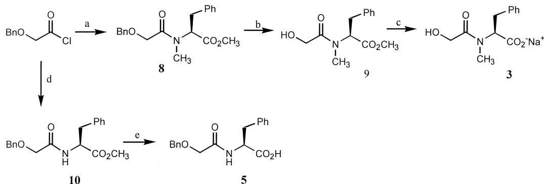
Scheme 3. Reagents and conditions: (a) N -Methyl-L-Phe-OCH 3 , Et 3 N, THF, 84%; (b) H 2 , Pd/C, MeOH, 90%; (c) 1N NaOH, MeOH, 90%; (d) L-Phe-OCH 3 -HCl, pyridine, THF, 75%; (e) 1N LiOH, MeOH, 95%.
