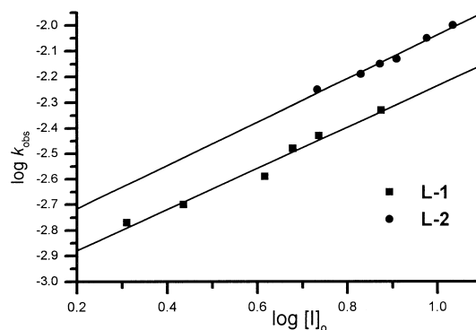
Figure 5. Determination of the reaction order in the inactivation of CPA by L-1 and L-2.
