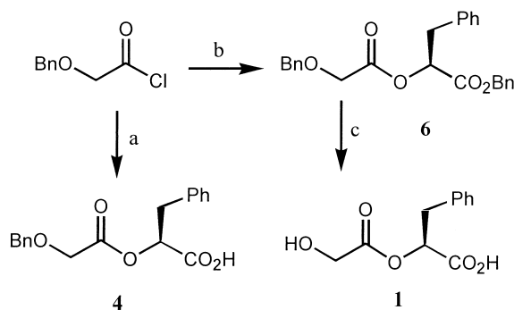
Scheme 1. Reagents and conditions: (a) L- \beta -Phenyllactic acid, pyridine, cat. DMAP, THF, 80%; (b) L- \beta -Phenyllactic acid benzyl ester, pyridine, THF, 81%; (c) \text{H}_2 , Pd/C (1 atm), MeOH, quant.
