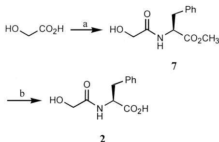
Scheme 2. Reagents and conditions: (a) L-Phe-OCH 3 , HCl, DCC, HOBT, NEM, THF, 45%; (b) 1N LiOH, MeOH, 90%.
