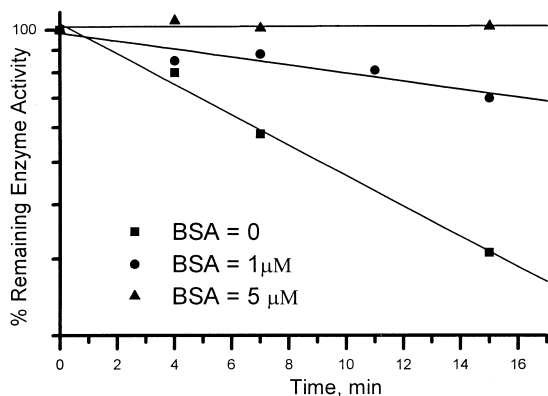
Figure 3. The rate of inactivation by L-1 was reduced by the presence of benzylsuccinic acid.
